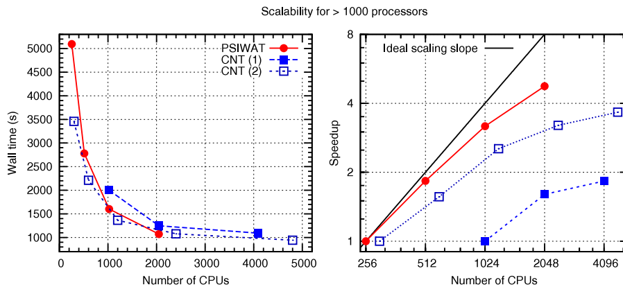
Figure 4. Scalability for large-scale calculations: wall time (left panel) and speedup (right panel) as a function of the number of processors. PSIWAT: PWscf code, n_{\text{pool}} = 4 , n_{\text{task}} = 4 , on a Cray XT 4. The system is a gold surface covered by thiols in interaction with water, 4 \mathbf{k} -points, 10.59 \times 20.53 \times 32.66 \text{ \AA}^3 cell, 587 atoms, 2552 electrons. CNT (1): PWscf code, n_{\text{task}} = 4 , on a Cray XT 4. The system is a porphyrin-functionalized nanotube, \Gamma point, 1532 atoms, 5232 electrons. CNT (2): CP code on a Cray XT3, same system as for CNT (1). Times for PSIWAT and CNT (1) are for 10 and 2 self-consistency iterations, respectively; times for CNT (2) are for 10 electronic steps plus 1 Car–Parrinello step, divided by 2 so that they fall in the same range as for CNT (1).
